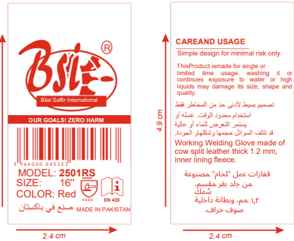
LABEL (WIDTH:2.4CM & LENGTH 4.9CM) (ONLY ON Left SIDE OF GLOVE) (LABEL COLOR :Red)
