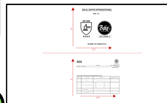
LABEL (WIDTH:3.8CM & LENGTH 5.08CM) (ON Both Left&Right Side of GLOVE) (LABEL COLOR :White )
